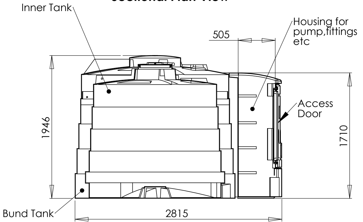
Sectional Elevation
